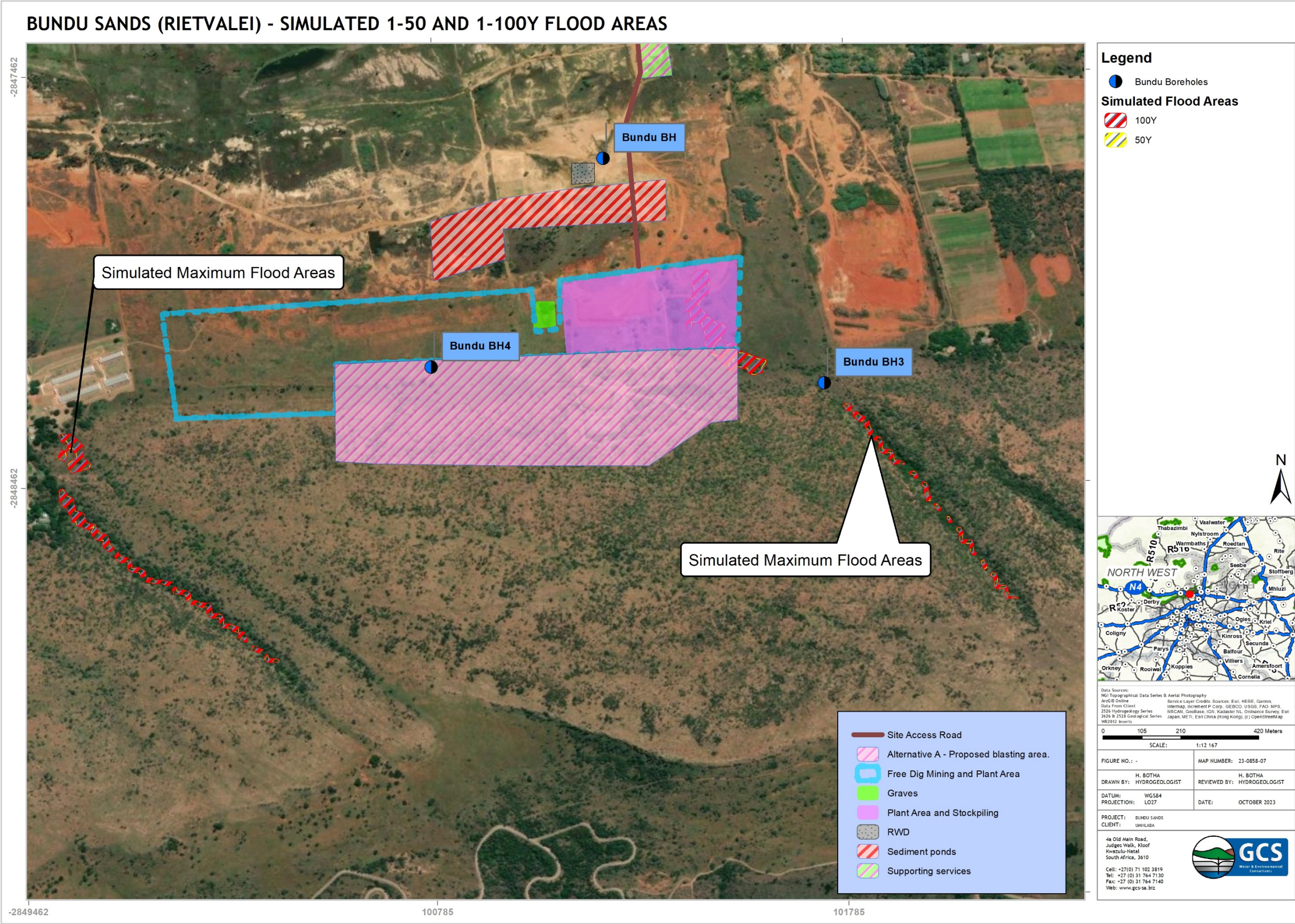
Figure 5-1: Simulated 1-50- and 1-100-year flooding areas for recognised drainage lines
