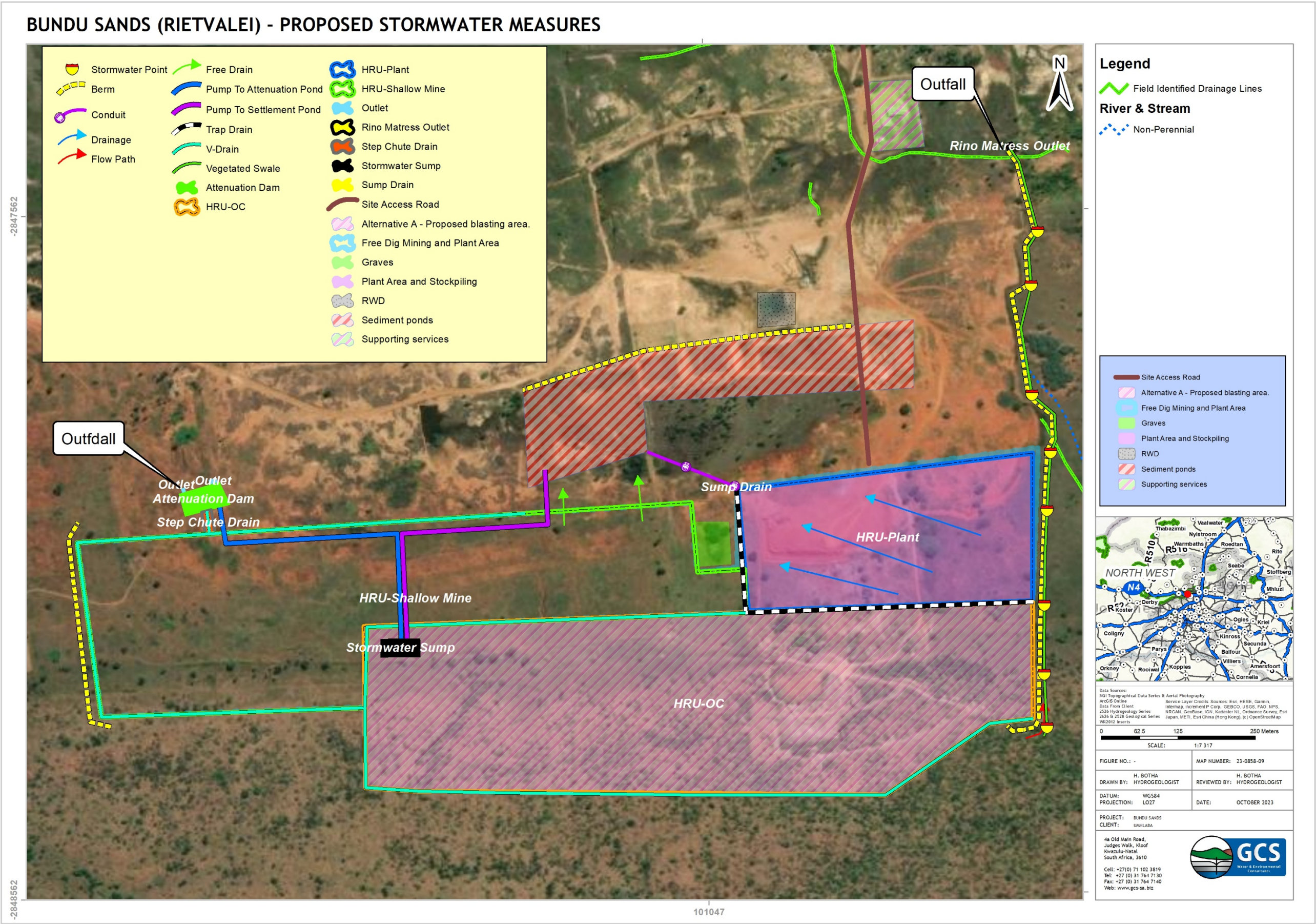
Figure 6-1: Stormwater catchments & proposed stormwater measures
