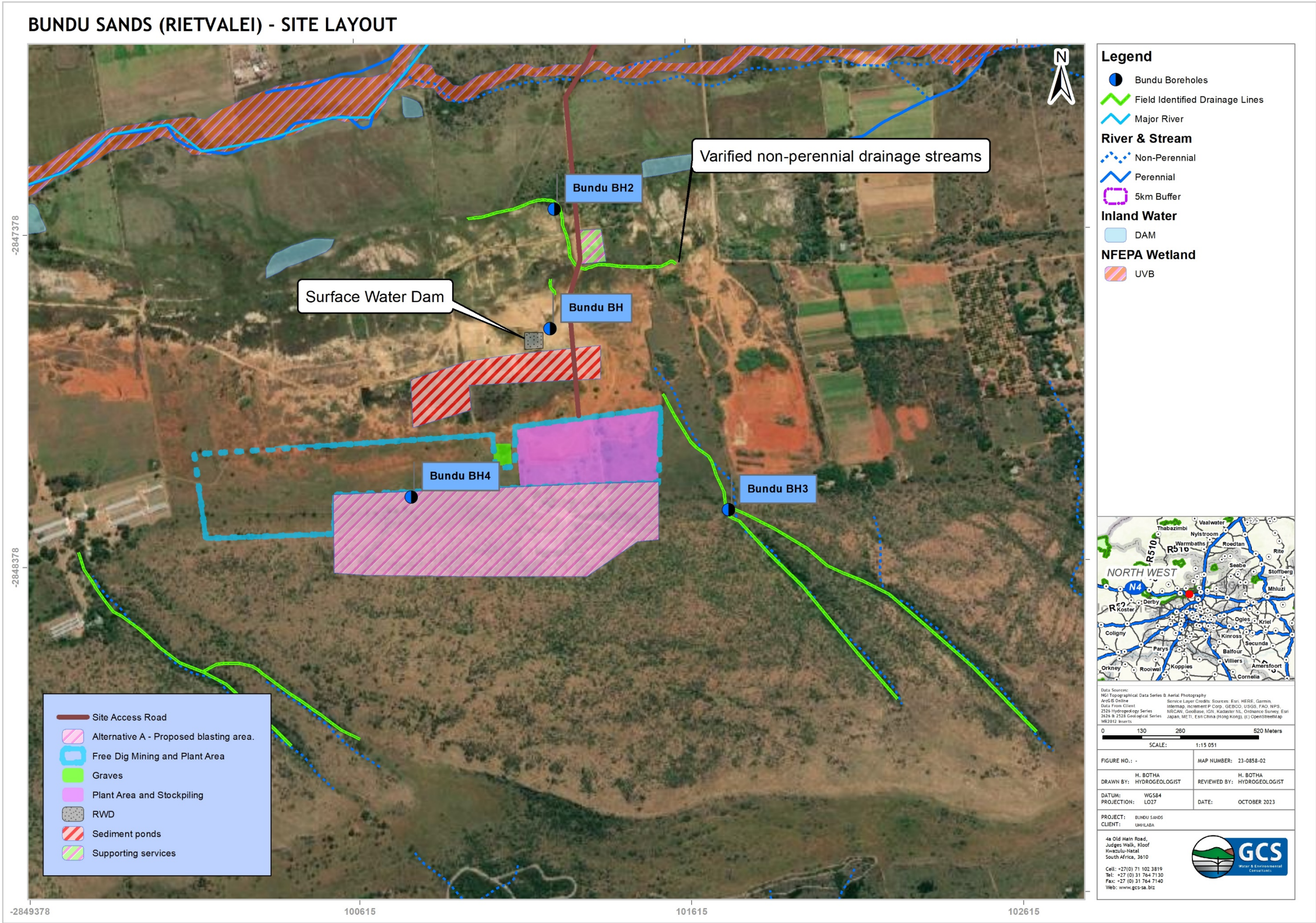
Figure 1-1: Site layout
