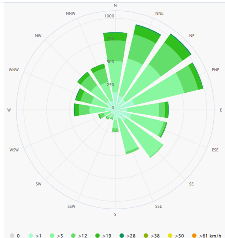
Figure 3-6: Wind rose (Meteoblue, 2023)
